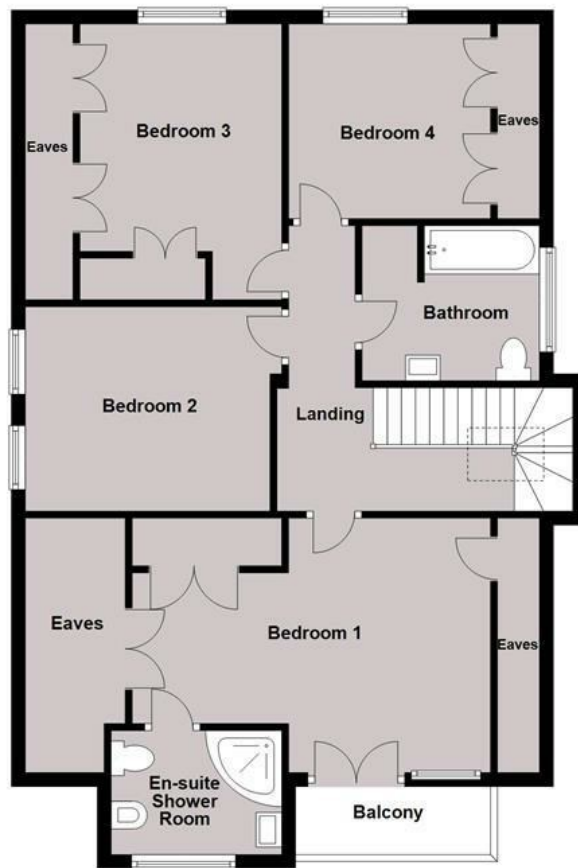
First Floor Approx. 84.2 sq. metres (905.8 sq. feet)
